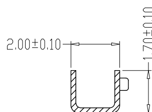
SEC:C-C
